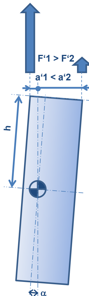
SITUATION 2: Load is inclined by 2,5^\circ
